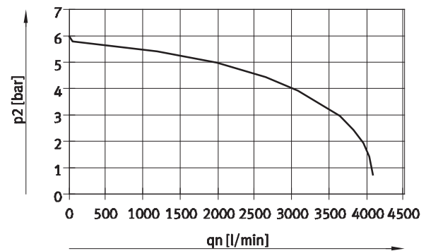
Flow rate q_n as a function of output pressure p_2 with pressure regulator plates (P regulator plate) for port 1 Supply pressure 10 bar, set control pressure 6 bar
