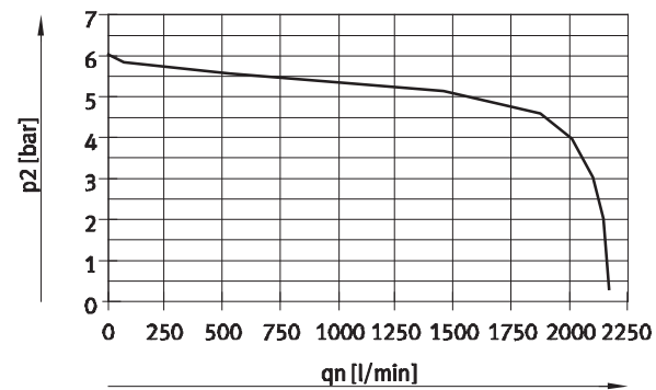
Flow rate q_n as a function of output pressure p_2 with pressure regulator plates (P regulator plate) for port 1 Supply pressure 10 bar, set control pressure 6 bar
